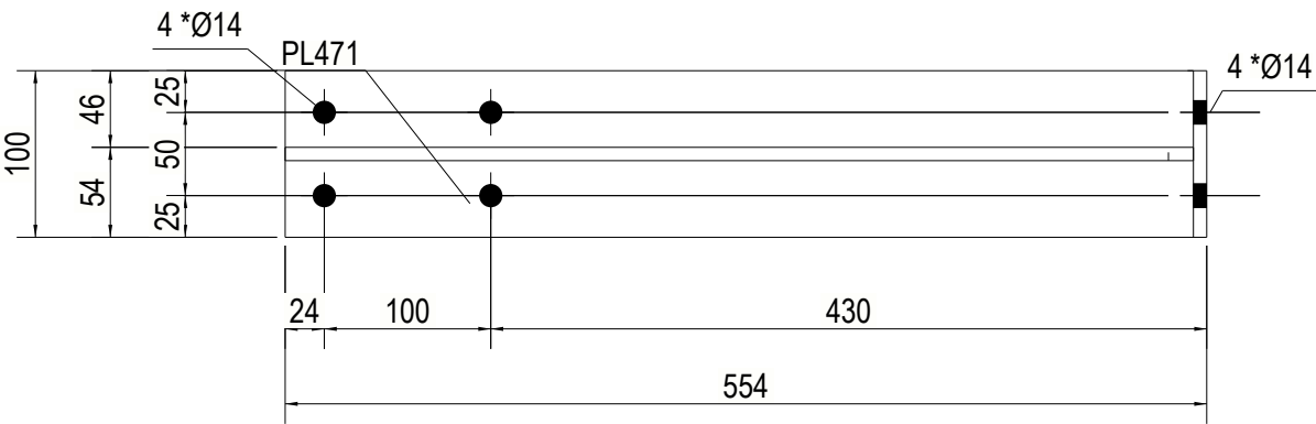
FRONT VIEW
